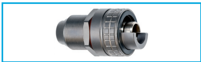
FWE Fixed socket, nut fixing (IP 68 when mated)
